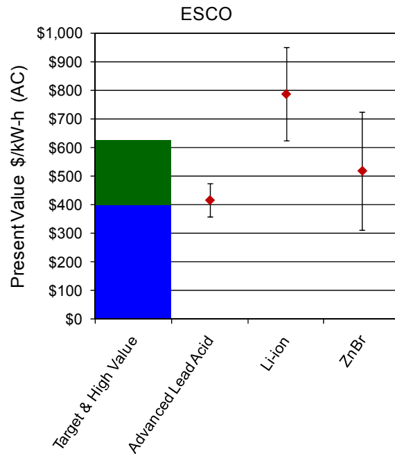
Figure A-9 ESCO Gap Chart
