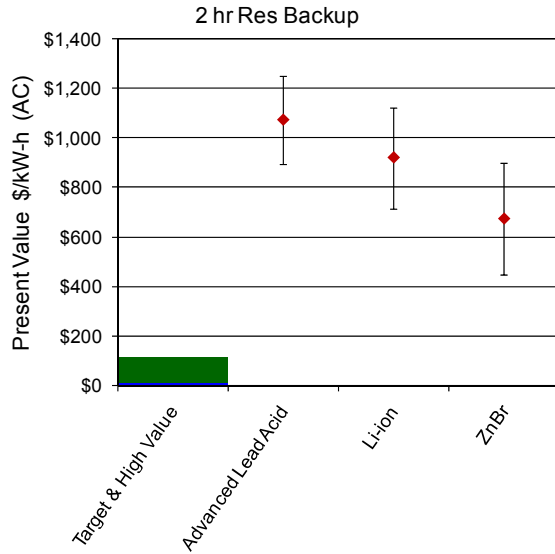
Figure A-8 Two-Hour Residential Backup Gap Chart
