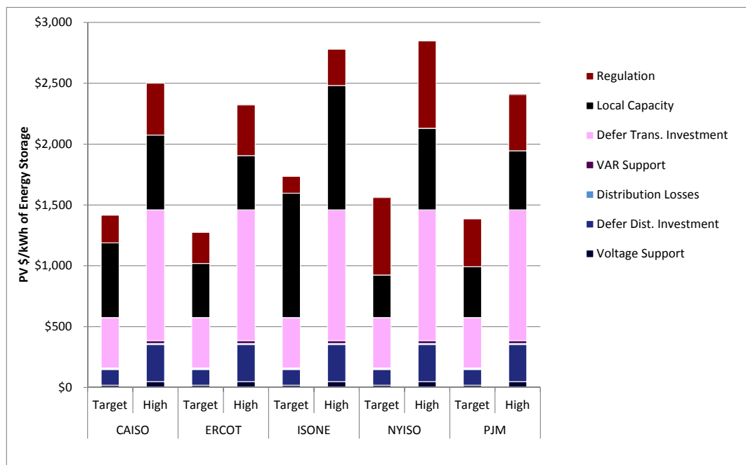
Figure 2-4 Stationary T&D Deferral, with Regulation and Transmission Deferral
