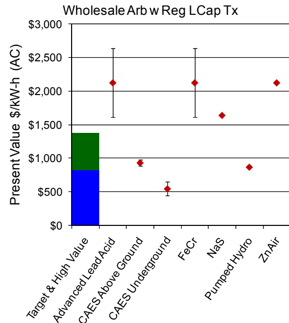
Figure A-23 Wholesale Energy Arbitrage with Regulation, Local Capacity, and Transmission Benefit Values Gap Chart
