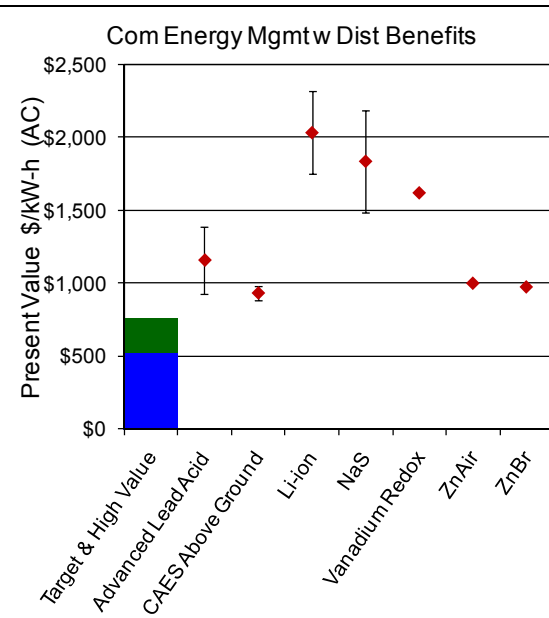
Figure A-16 Commercial Energy Management with Distribution Benefits Gap Chart
