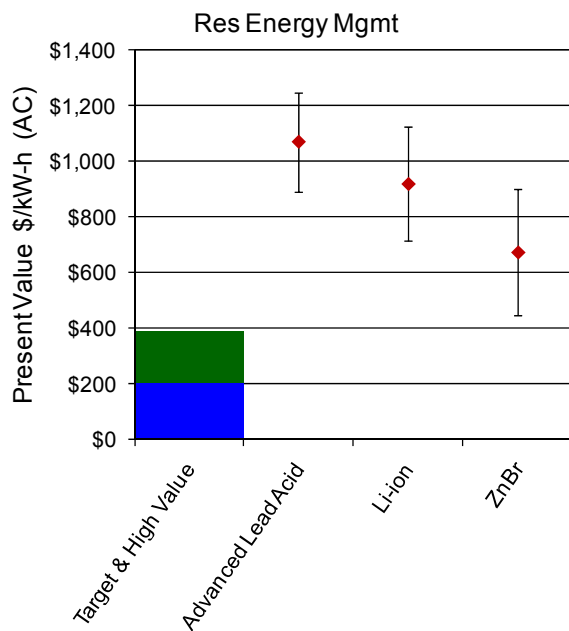
Figure A-10 Residential Energy Management Gap Chart
