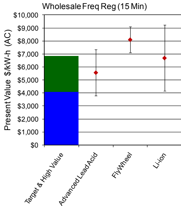
Figure A-21 Wholesale Frequency Regulation Gap Chart
