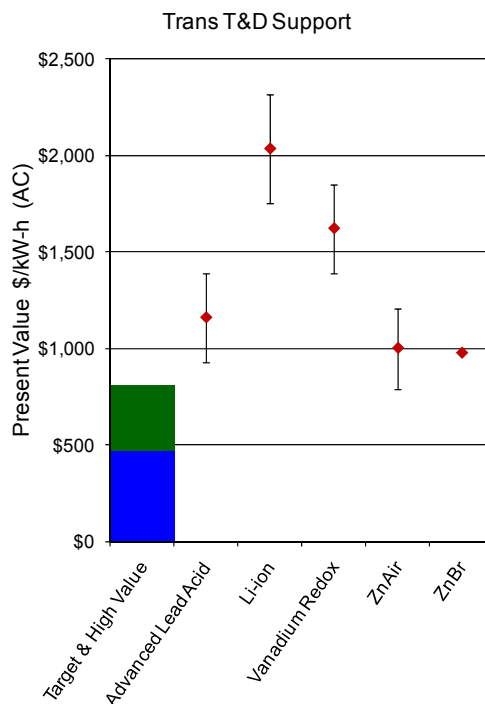
Figure A-19 Transportable Transmission and Distribution Support Gap Chart
