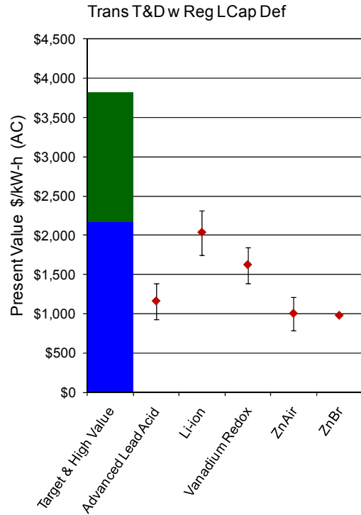
Figure A-20 Transportable Transmission and Distribution with Regulation, Local Capacity and Deferral Benefit Values Gap Chart
