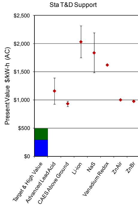
Figure A-17 Stationary Transmission and Distribution Support Gap Chart
