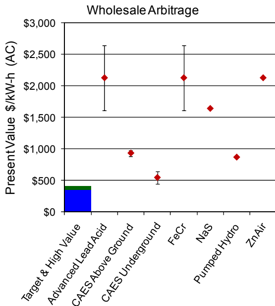
Figure A-22 Wholesale Energy Arbitrage Gap Chart
