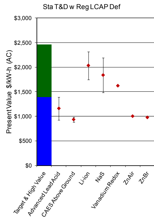
Figure A-18 Stationary Transmission and Distribution Support with Regulation, Local Capacity and Deferral Benefit Values Gap Chart
