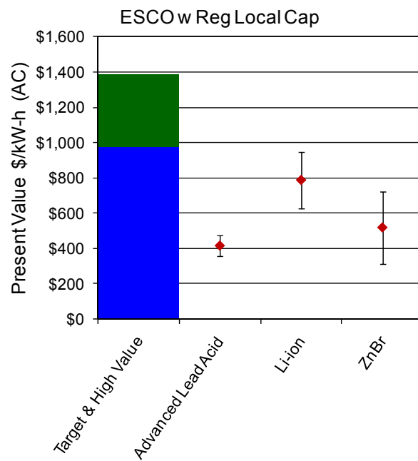
Figure A-11 ESCO with Regulation and Local Capacity Benefit Values Gap Chart
